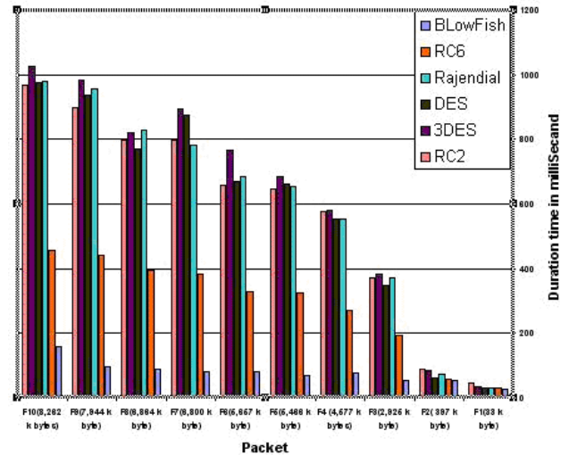
Figure 7: Time consumption for encrypt different audio files
